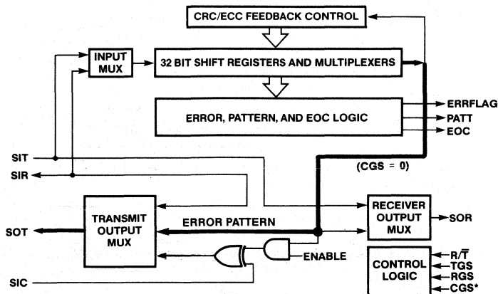
Figure 8a. Data Flow in the SiBER for Hardware/Software Correction
