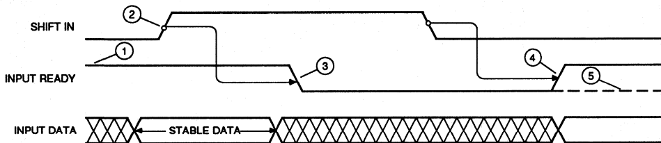
Figure 1. Input Timing
