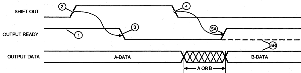
Figure 4. Output Timing
