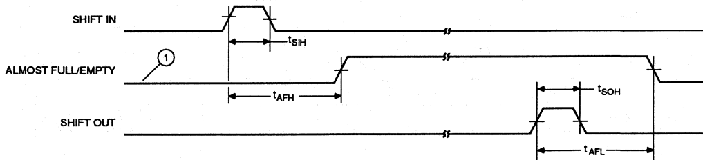
Figure 9. t_{AEH} , t_{AEL} Specifications
