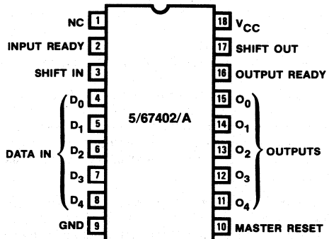
Figure 4. 67402 Pinout
