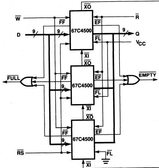
Figure 12. Depth-Expansion to Form a 768x9 FIFO
