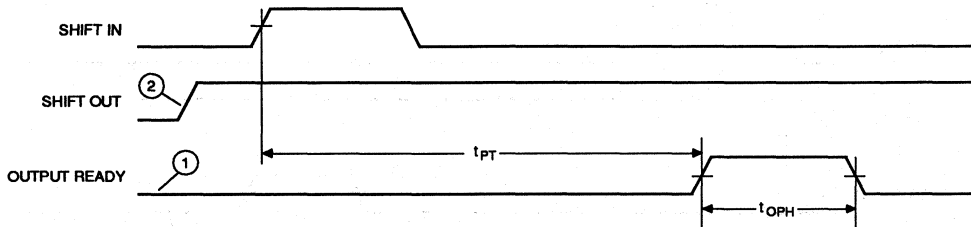
Figure 5. The Mechanism of Shifting Data Out of the FIFO
