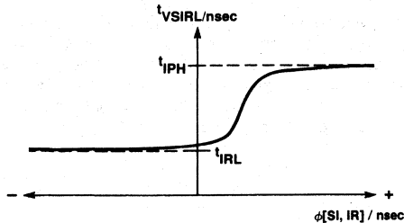
Figure 9. t_{VSIRL} as a Function of Phase
