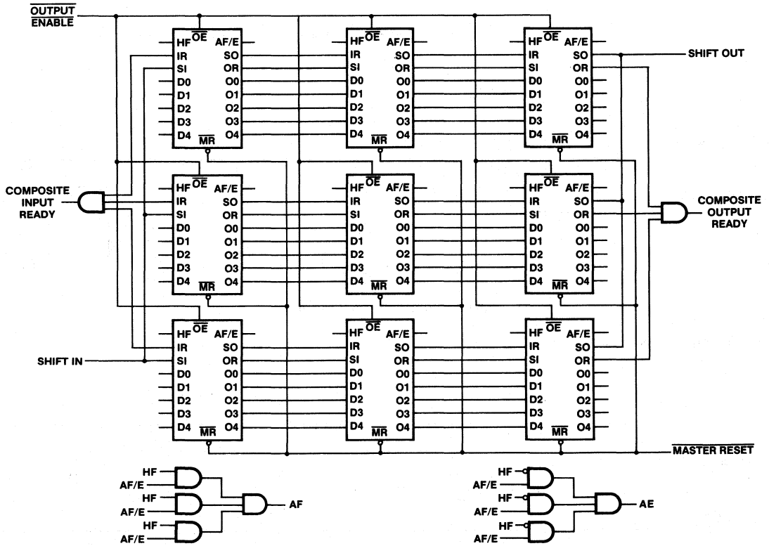
The First Column of FIFOs
