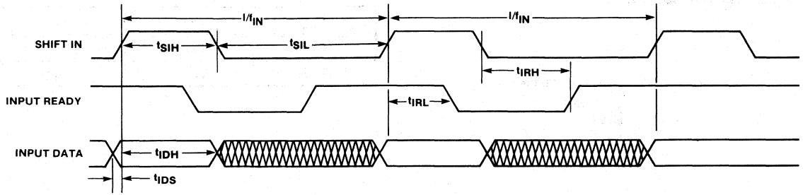
Figure 1. Input Timing
