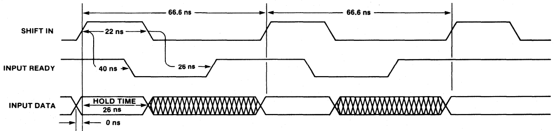
Figure 2. Typical Waveforms for 15-MHz Shift-In Rate
