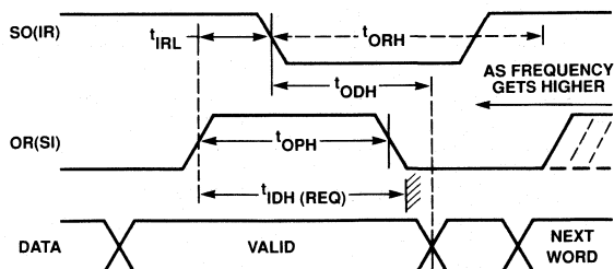
Figure 6. Higher-Frequency Fallthrough
