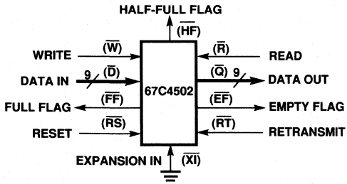
Figure 10. Single FIFO Configuration
