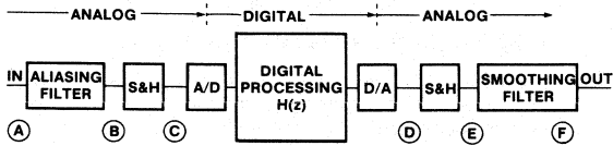
Figure 3. DSP Functions
