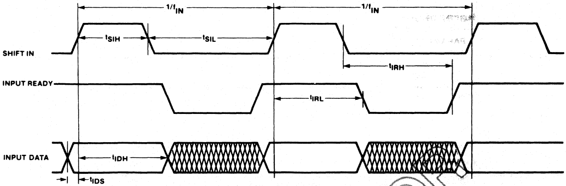
Figure 1. Input Timing
