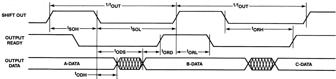
Figure 5. Output Timing
