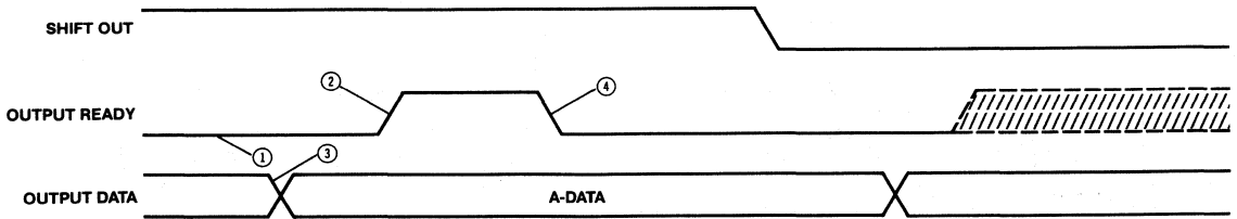
Figure 9. Data is Shifted Out Whenever Shift Out and Output Ready are Both HIGH
