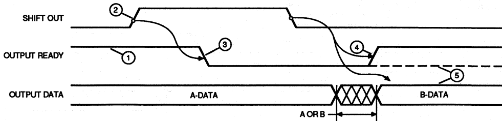
Figure 4. Output Timing
