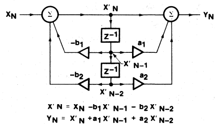
Figure 5. Digital Biquadratic Filter Section
