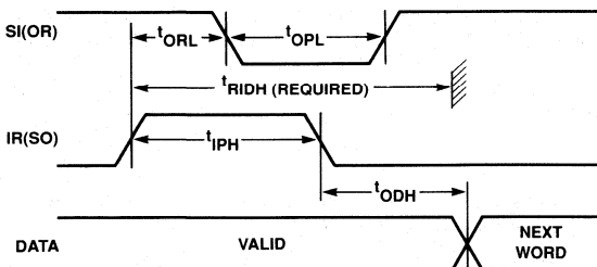
Figure 5. Low-Frequency Bubbleback
