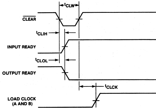
Figure 6. Clear Timing
