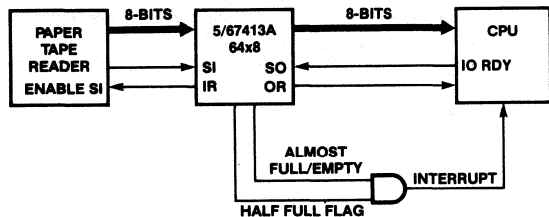
Figure 1. Slow Steady Rate to Fast 'Blocked Rate' FIFO Applications
