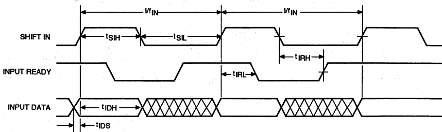
Figure 1. Input Timing
