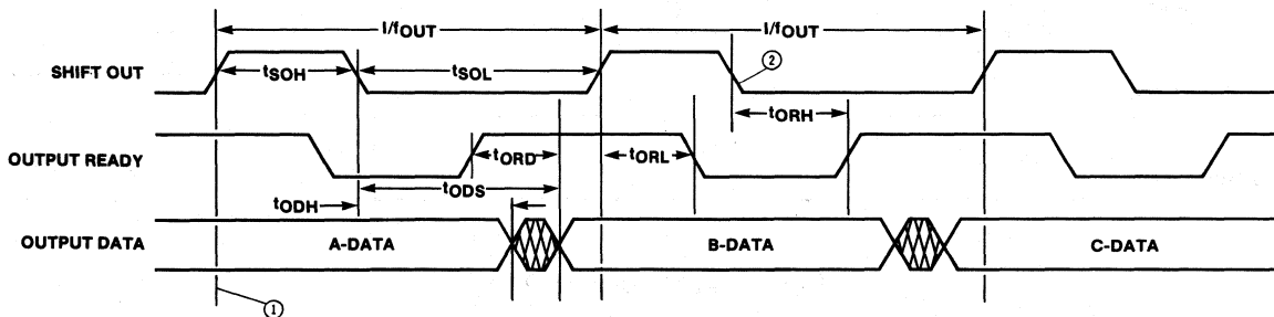
Figure 5. Output Timing
