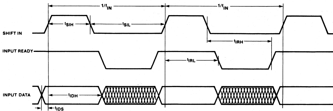
Figure 1. Input Timing
