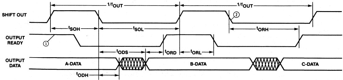
Figure 4. Output Timing
