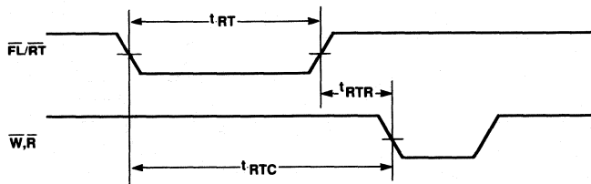
Figure 7. Retransmit Timing
