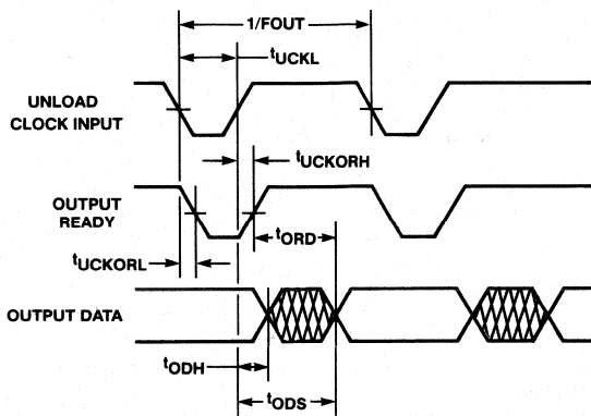
Figure 4. Output Timing
