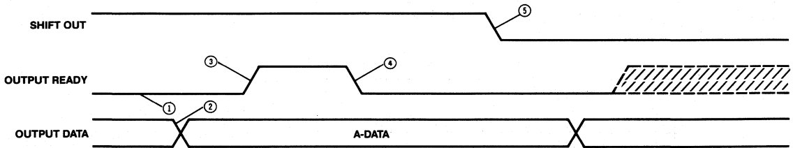
Figure 7. Data is Shifted Out Whenever Shift Out and Output Ready are Both HIGH
