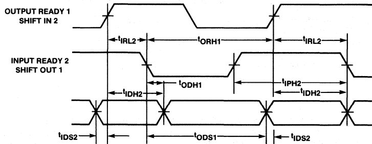
Figure 20. Handshake Timing
