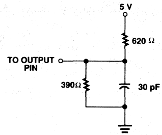
Figure 15. A.C. Test Load
