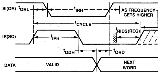
Figure 7. Higher-Frequency Bubbleback
