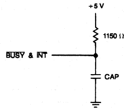
Test Loads C and D
