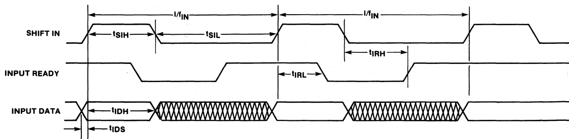
Figure 1. Input Timing
