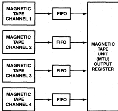
Figure 13. Magnetic Tape Lead to MTU Output
