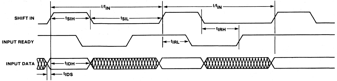
Figure 1. Input Timing
