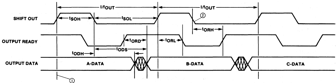
Figure 5. Output Timing
