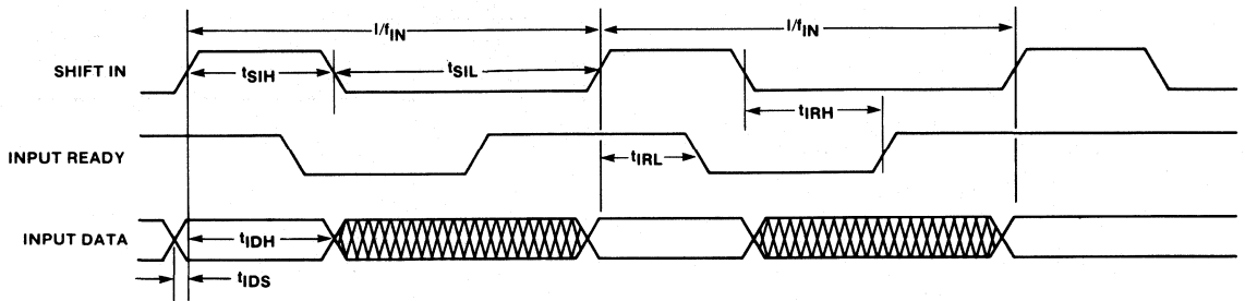
Figure 1. Input Timing
