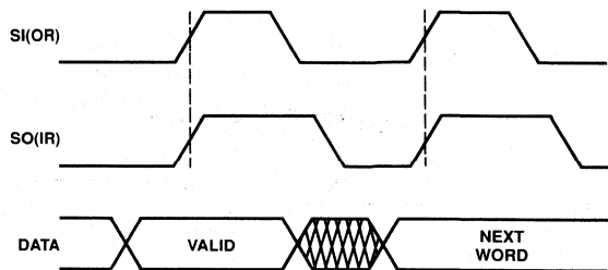
Figure 8. Zero-Phase Incidence
