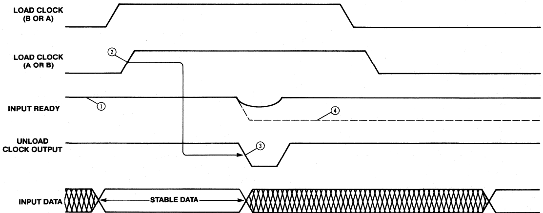
Figure 2. Input Timing
