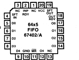
Plastic Chip Carrier
