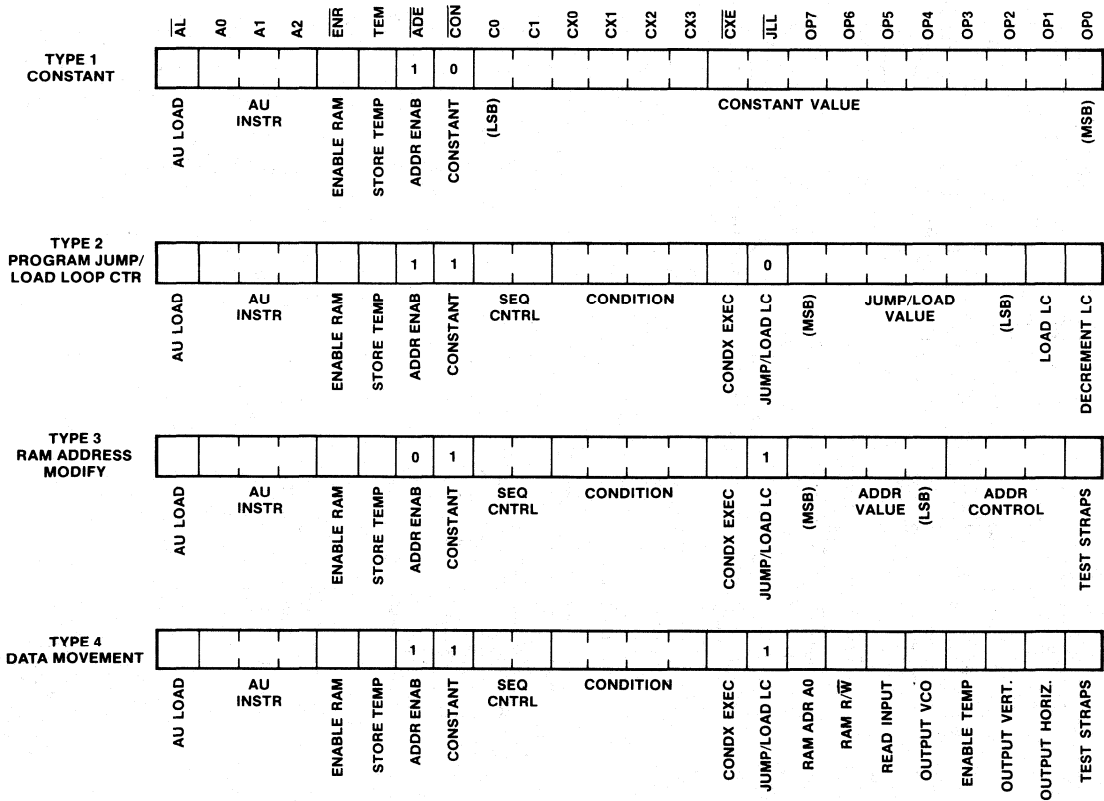
Figure 12. Microinstruction Word Formats
