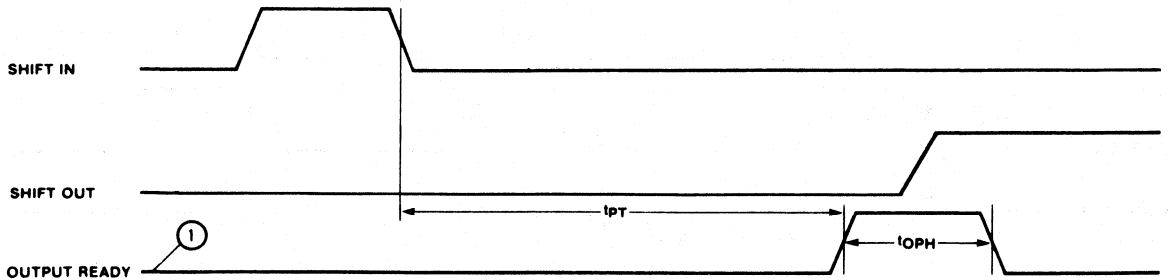
Figure 8. t_{PT} and t_{OPH} Specification
