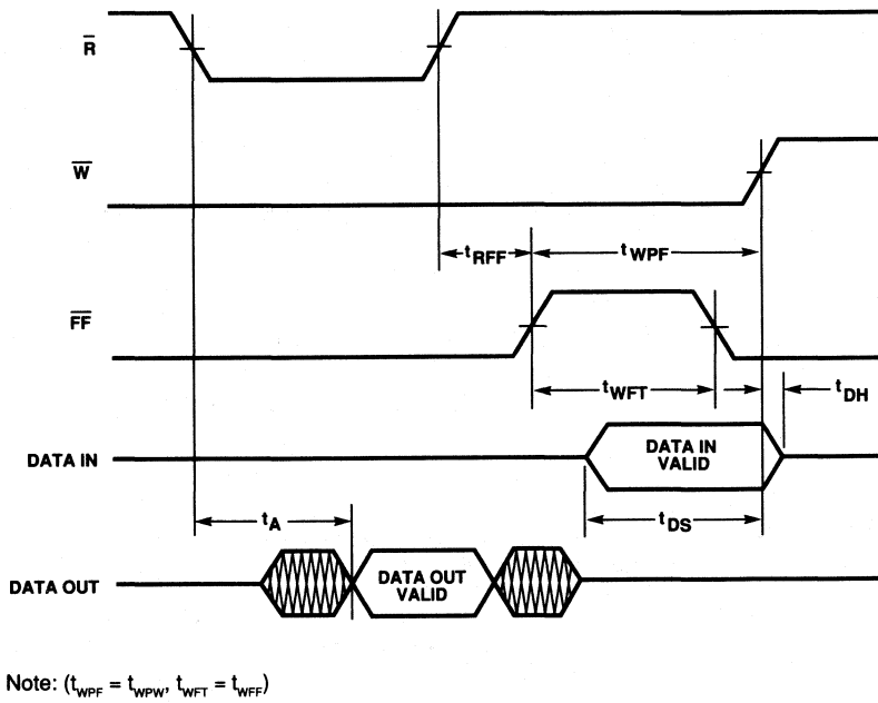
Figure 8. Read Data Flow Through Mode
