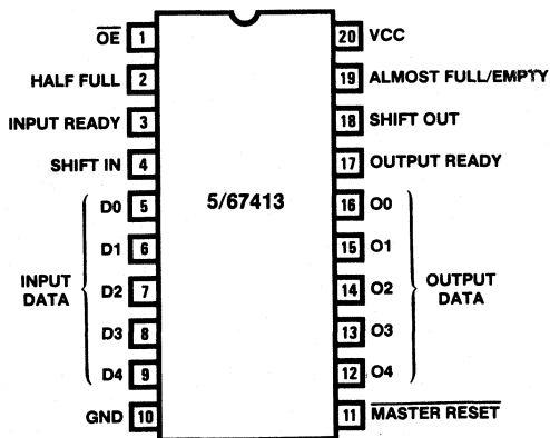
Figure 2. 67413 Pin Configuration
