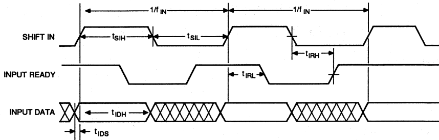
Figure 1. Input Timing
