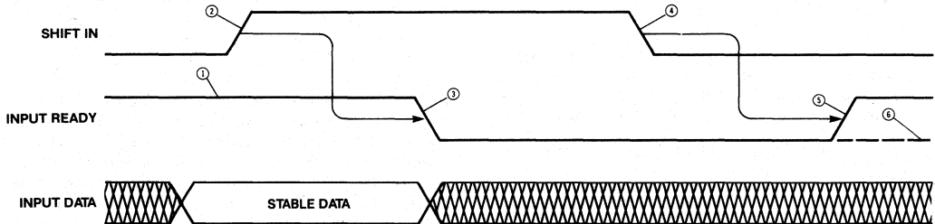
Figure 16. The Mechanism of Shifting Data Into the FIFO
