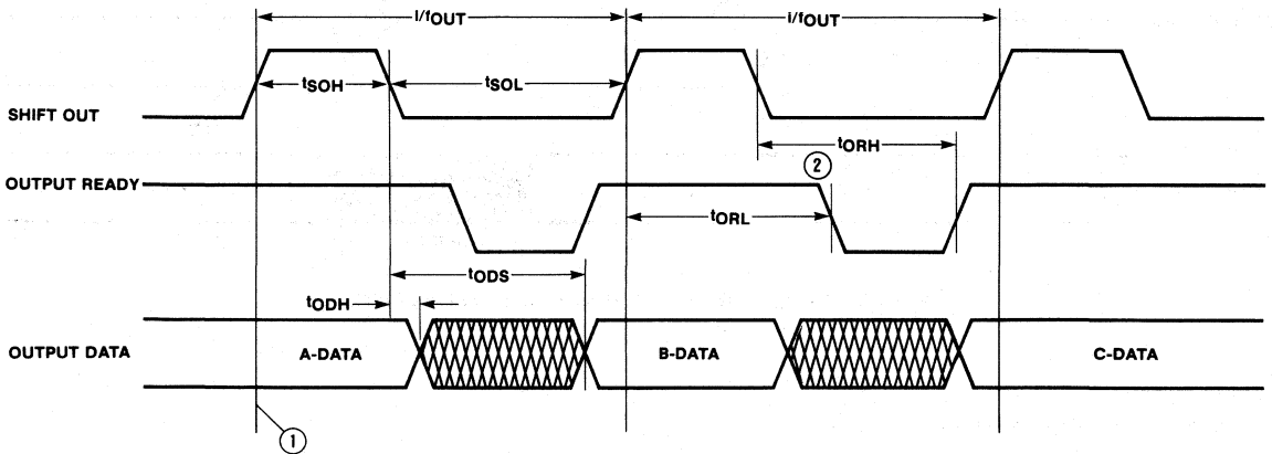
Figure 5. Output Timing
