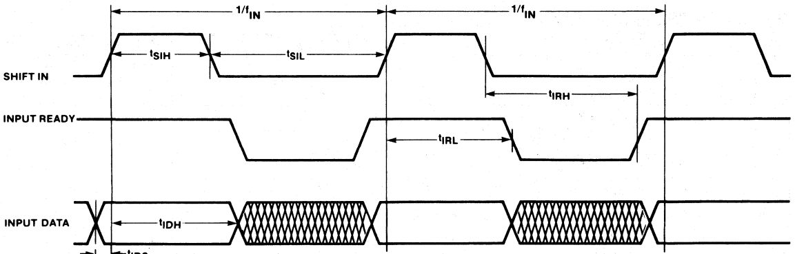
Figure 1. Input Timing
