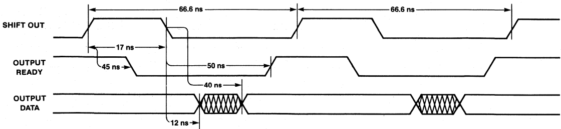
Figure 6. Typical Waveforms for 15 MHz Shift-Out Data Rate
