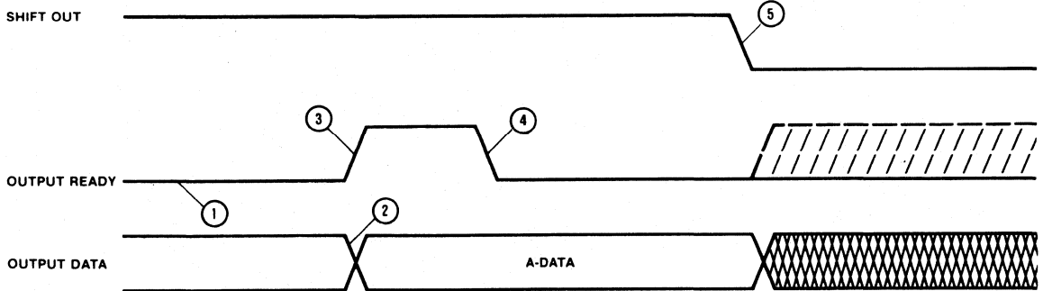
Figure 9. Data is Shifted Out Whenever Shift Out and Output Ready are Both HIGH.
