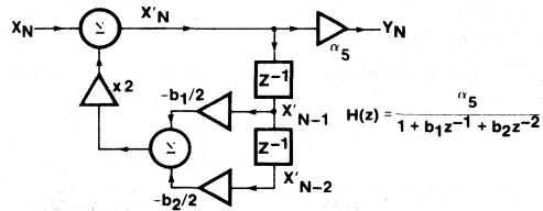
Figure 8. All-Pole Digital Filter Section
