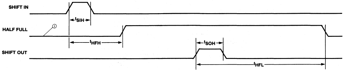
Figure 12. t_{HFL} , t_{HFH} Specifications
