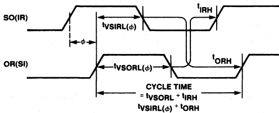
Figure 10. Positive SO/OR Phase at Natural Frequency
