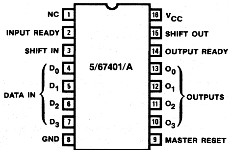
Figure 3. 67401/3341 Pinout
