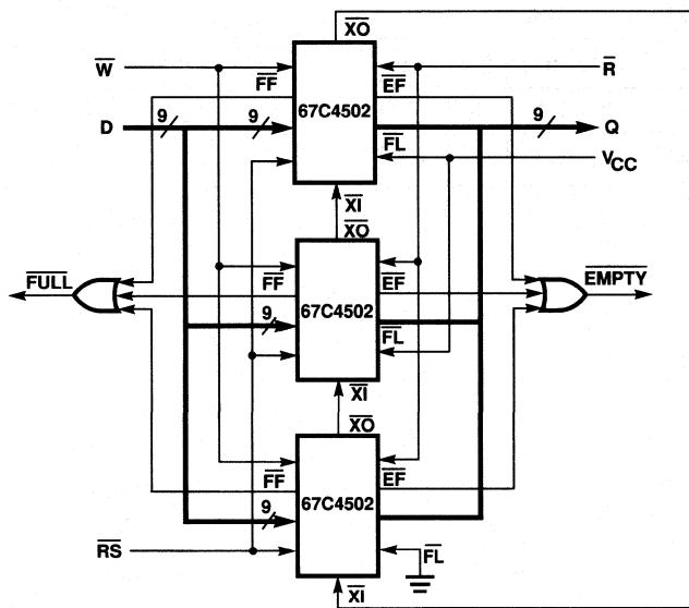
Figure 12. Depth-Expansion to Form a 3072x9 FIFO
