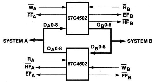
Figure 14. Bidirectional FIFO Mode
