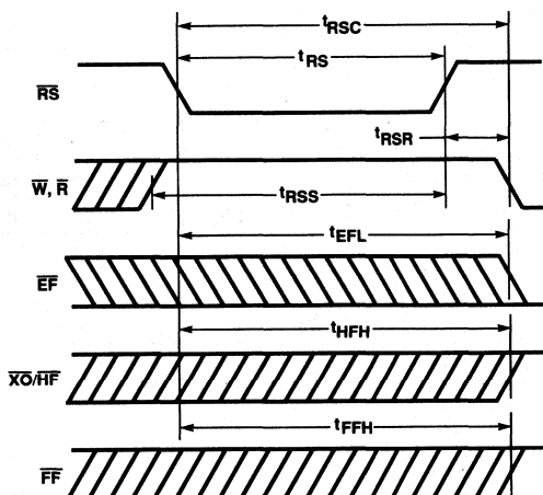
Figure 2. Reset Timing
