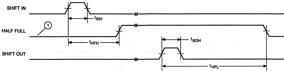
Figure 11. t_{HFL} , t_{HFH} Specifications
