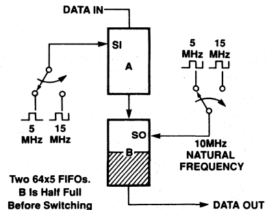
Figure 12. Approach of f_{MAX} from Fallthrough
