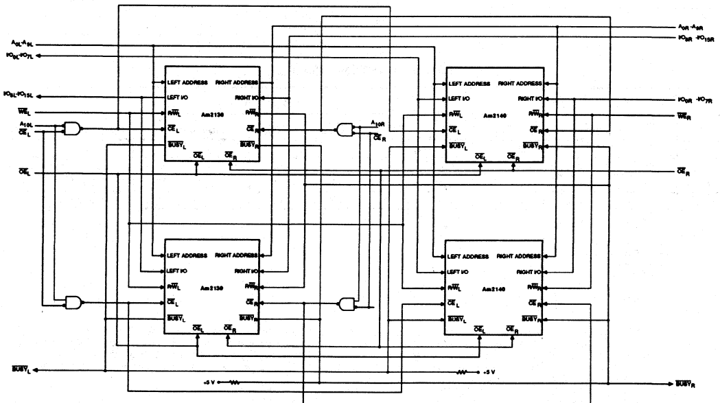
Figure 5. Conceptual Diagram of a 2K x 16 System Using Master/Slave
