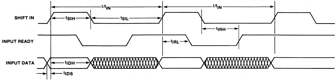
Figure 1. Input Timing
