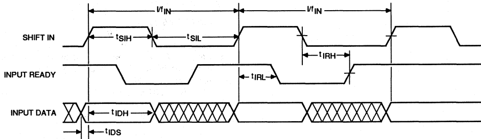
Figure 1. Input Timing
