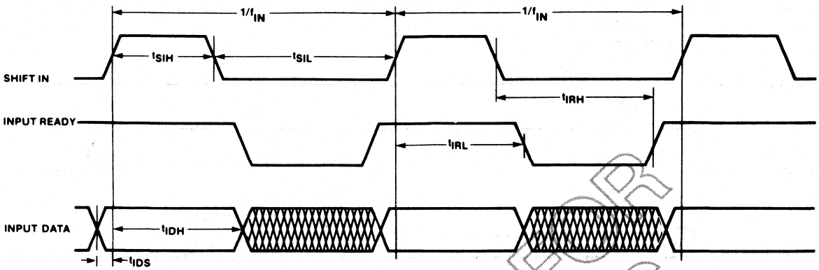
Figure 1. Input Timing
