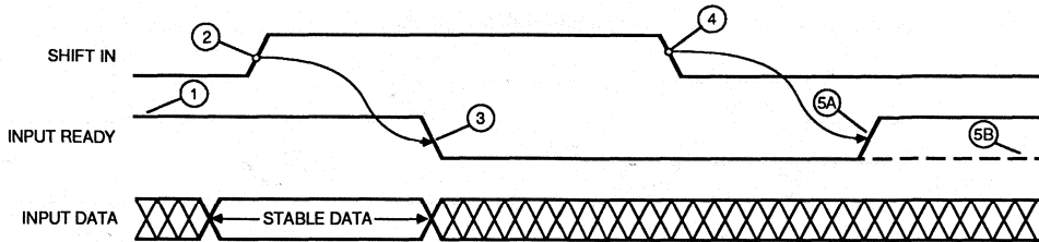
Figure 1. Input Timing
