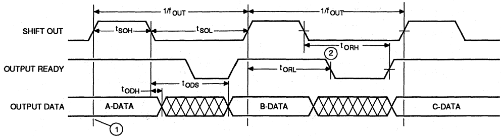
Figure 4. Output Timing
