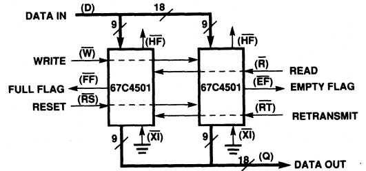
Figure 11. Width-Expansion to Form a 512x18 FIFO
