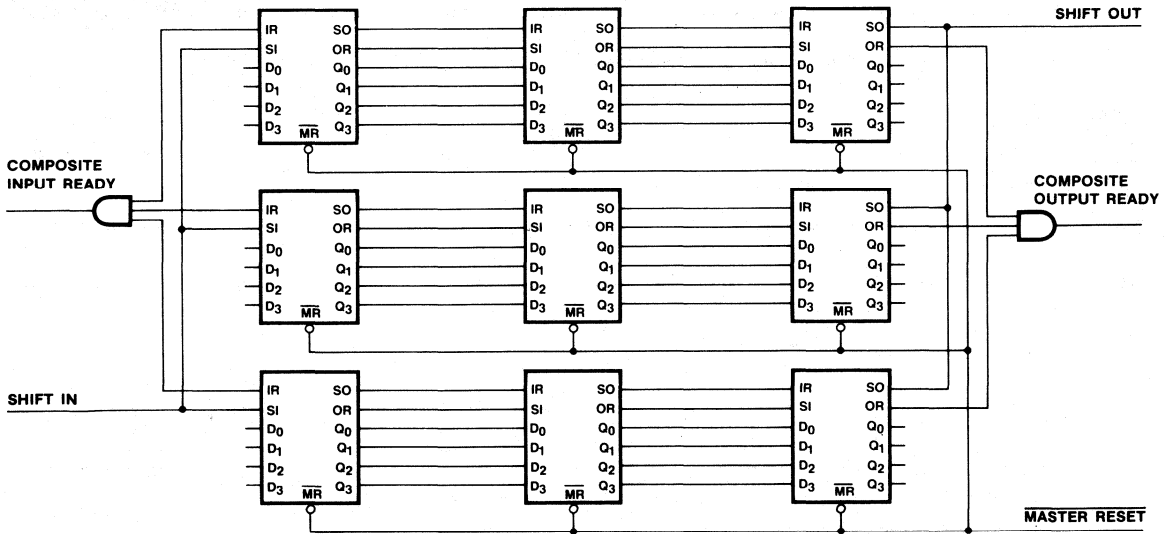
Figure 12. 192x12 FIFO with C5/C67401A/1B
