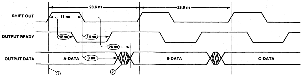
Figure 6. Typical Waveforms for 35 MHz Shift-Out Data Rate
