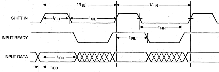
Figure 1. Input Timing
