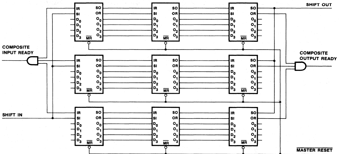
Figure 6. 192x12 FIFO
