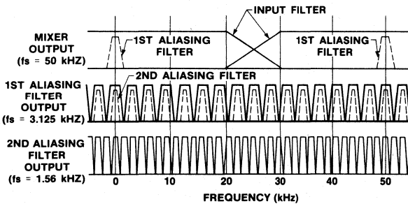
Figure 9. Aliasing Spectra for f_s Reduction
