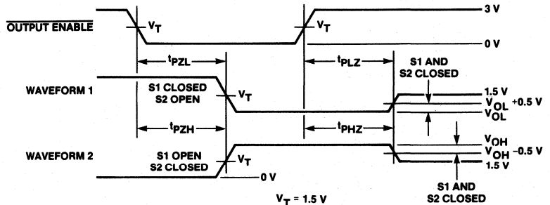
Figure A. Enable and Disable
